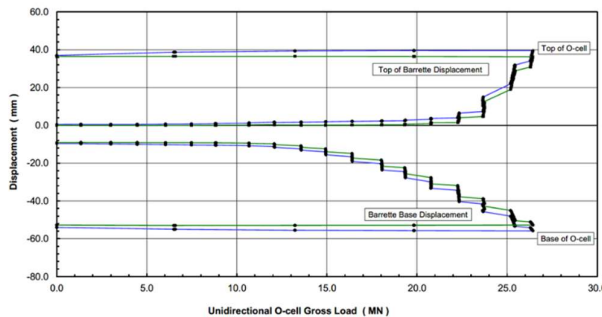
Fig. 7. Load - displacement top and base of O-cell movement.
