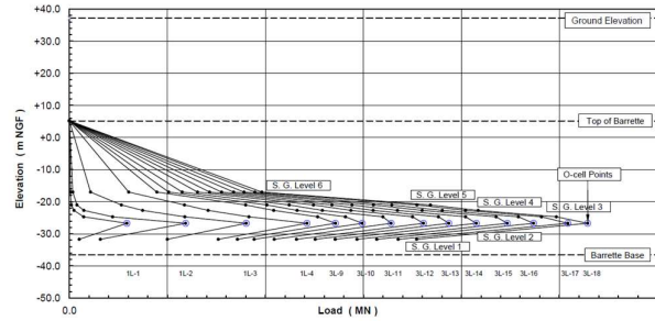
Fig. 8. Strain gauge (SG) load distribution.
