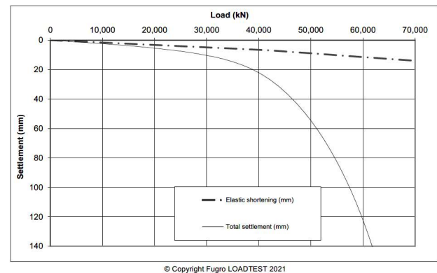
Fig. 9. Total Load-Settlement behavior.
