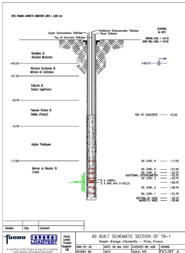
Fig. 3. Schematic section of the test barrette with strain gauges (SG) levels in relation to the soil conditions.
