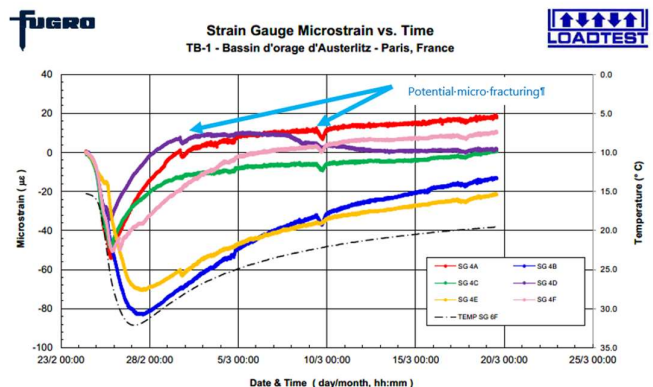
Fig. 5. Strain Gauge Microstrain v. Time with signs of potential micro fracturing.
