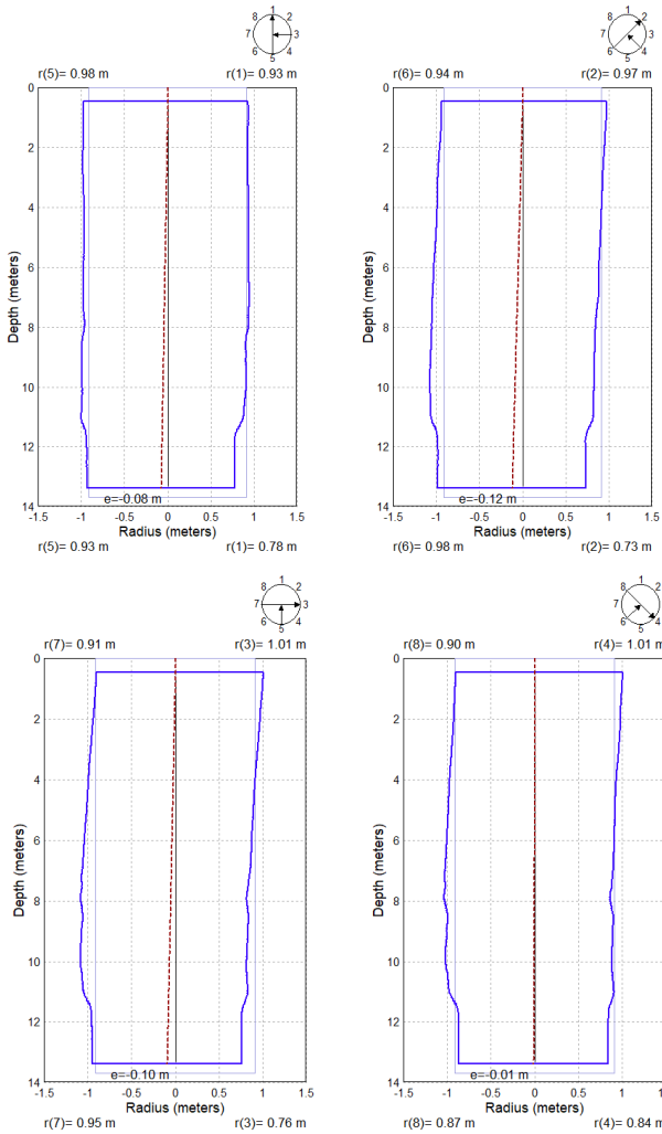
Fig 4. N-S (5-1), NE-SW (6-2), E-W (7-3), and SE-NW (8-4) profiles of radius vs depth through excavation.
