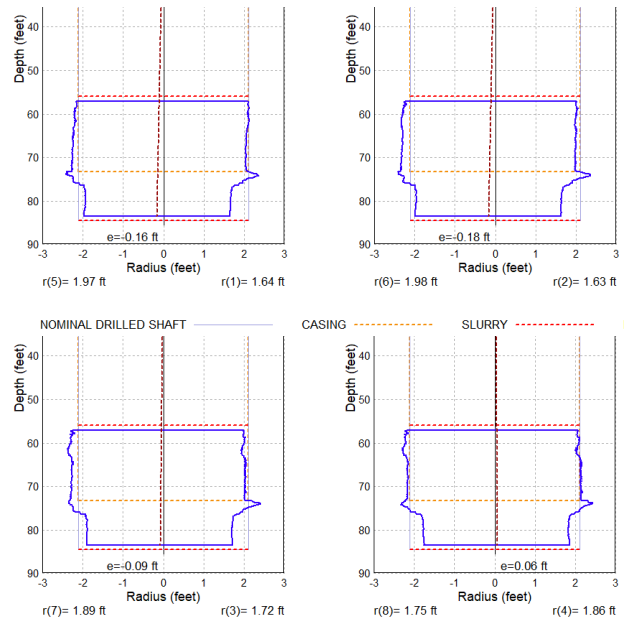
Fig. 6. SHAPE test results from shaft with caving soil below casing.
