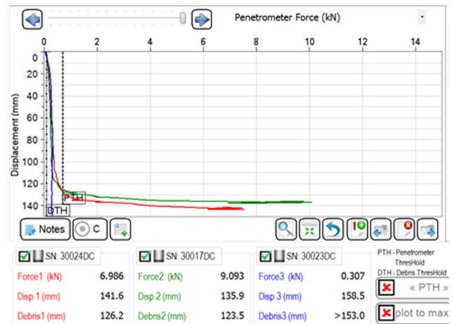
Fig. 8a. SQUID results from shale bedrock exposed to drilling fluid for four days
