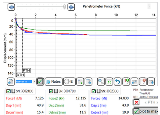
Fig. 8b. SQUID results from shale bedrock re-drilled and cleaned by air lifting
