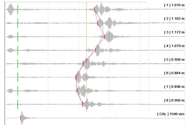
Fig 2. Ultrasonic signals at one test depth.
