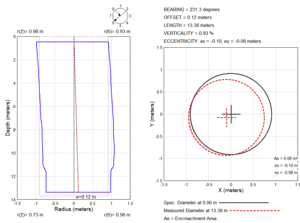
Fig 5. Maximum calculated eccentricity and resulting excavation verticality.
