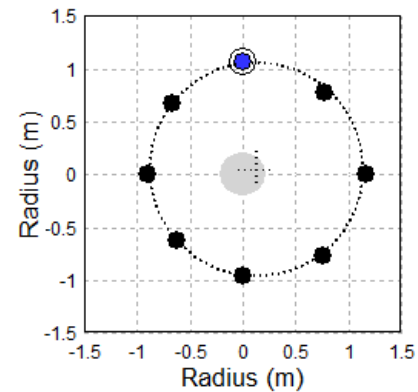
Fig 3. X-Y plot of excavation at the selected depth in relation to the top of shaft centroid
